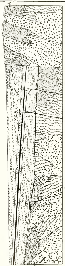
Figure 7. CLOSE OF THE TRIASSIC BASIN
